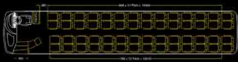
LAYOUT OF MCV S140R | 58 RECLINING PASSENGER SEATS + DRIVER
